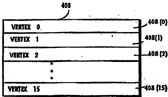
VERTEX BUFFER
